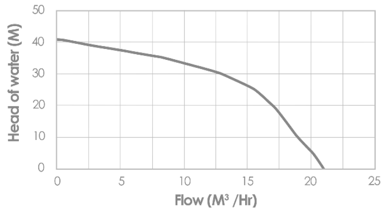
50mm High Head Borehole
